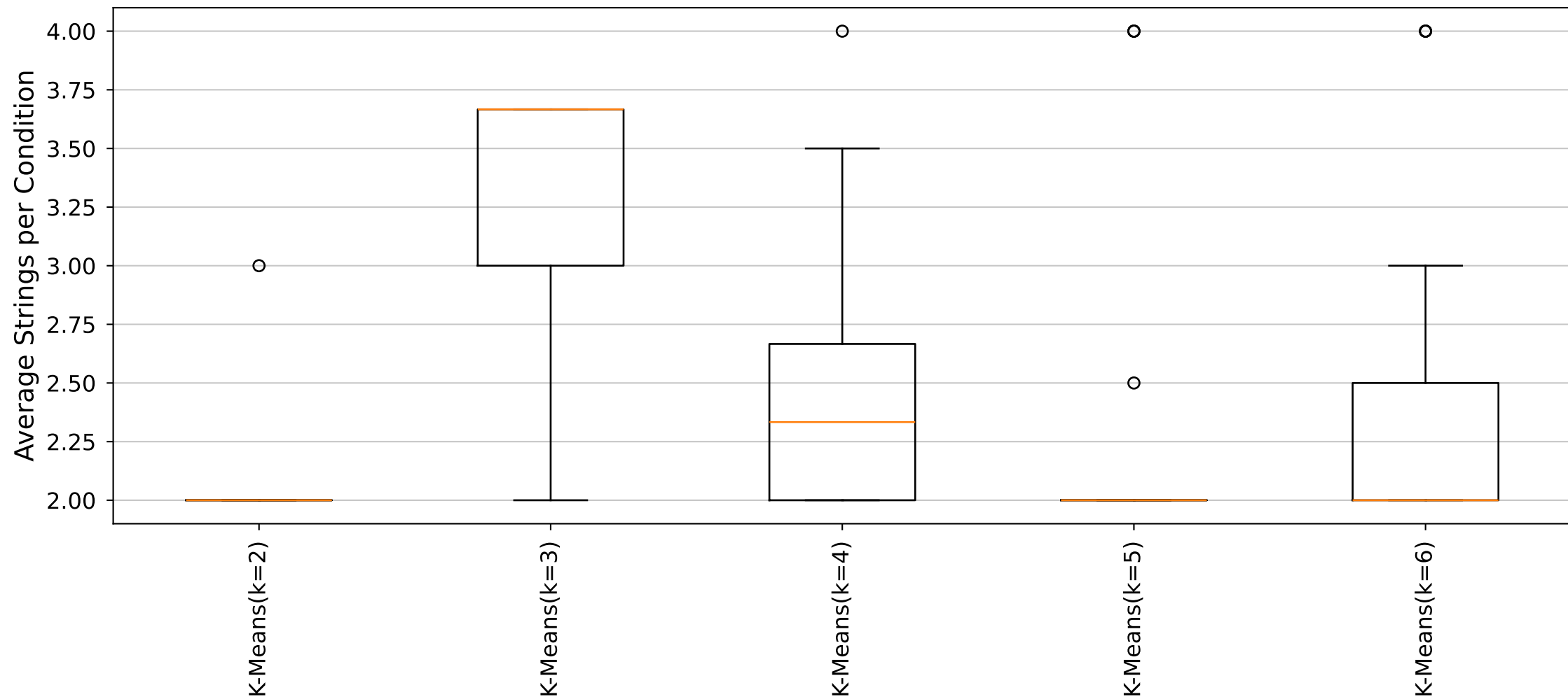
YARA Rules Average Strings per Condition Distribution (Cluster26_Size6 dataset)
